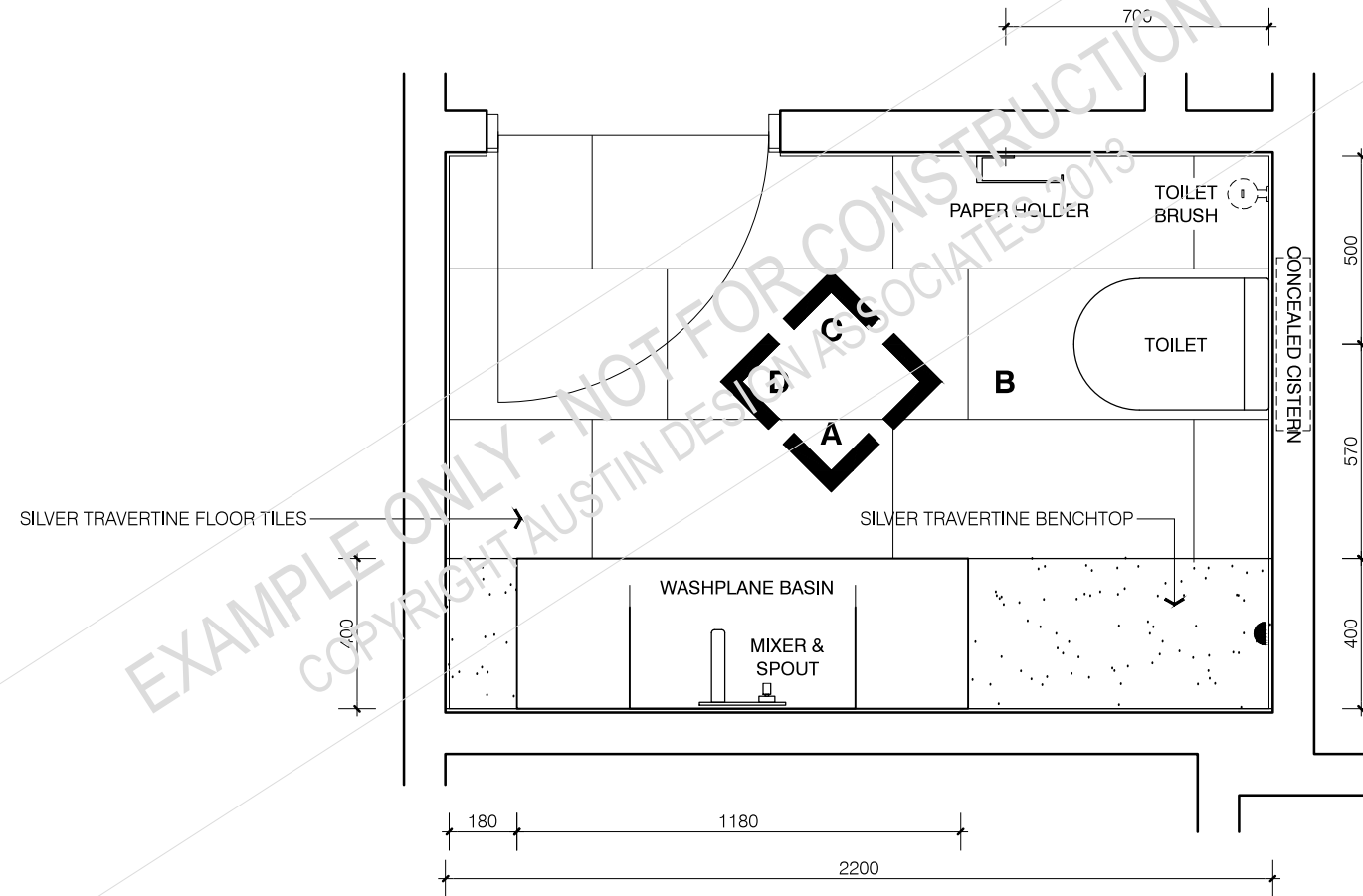
FF POWDER ROOM PLAN
